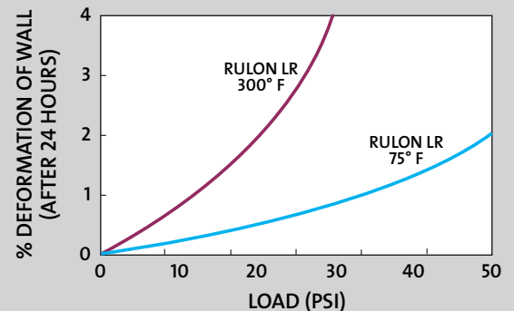
FIGURE K: DEFORMATION VS. LOAD
