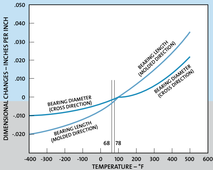
FIGURE O: EXPANSION OF RULON LR VS. TEMP
