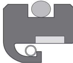
Lipseals sizes according to DIN 3760
